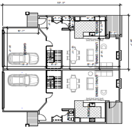
UNIT B - 1ST FLOOR PLAN 12' 0" x 12' 0"
