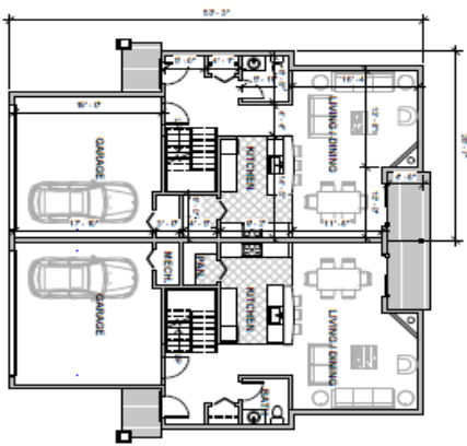
UNIT A - 1ST FLOOR PLAN 1/8" = 1'-0"
