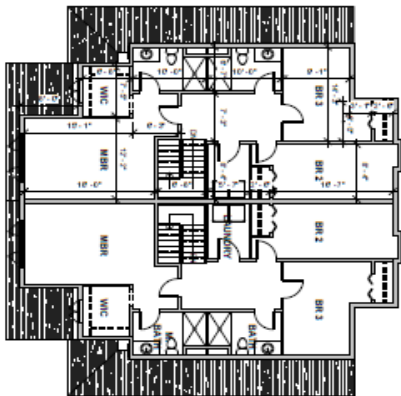
UNIT B - 2ND FLOOR PLAN 12' 0" x 12' 0"
