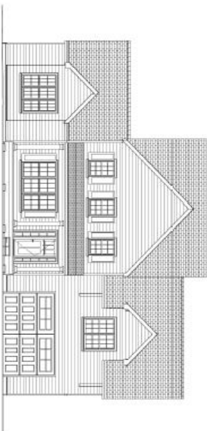
FRONT ELEVATION
