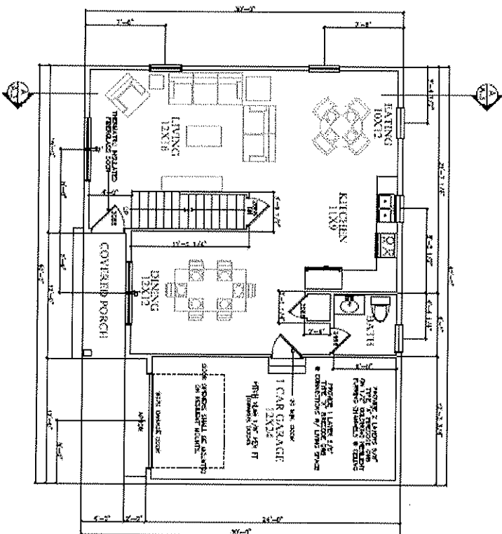
PROPOSED FIRST FLOOR PLAN 758 SF
