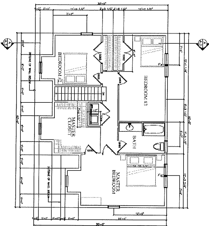
PROPOSED SECOND FLOOR PLAN 1,022 SF
